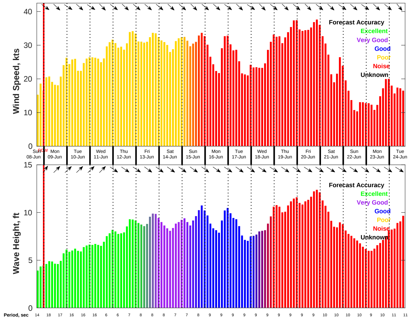
Wind & Wave Forecast for NDBC 46028 from 08-Jun-2025 16:00:00 to 24-Jun-2025 16:00:00
