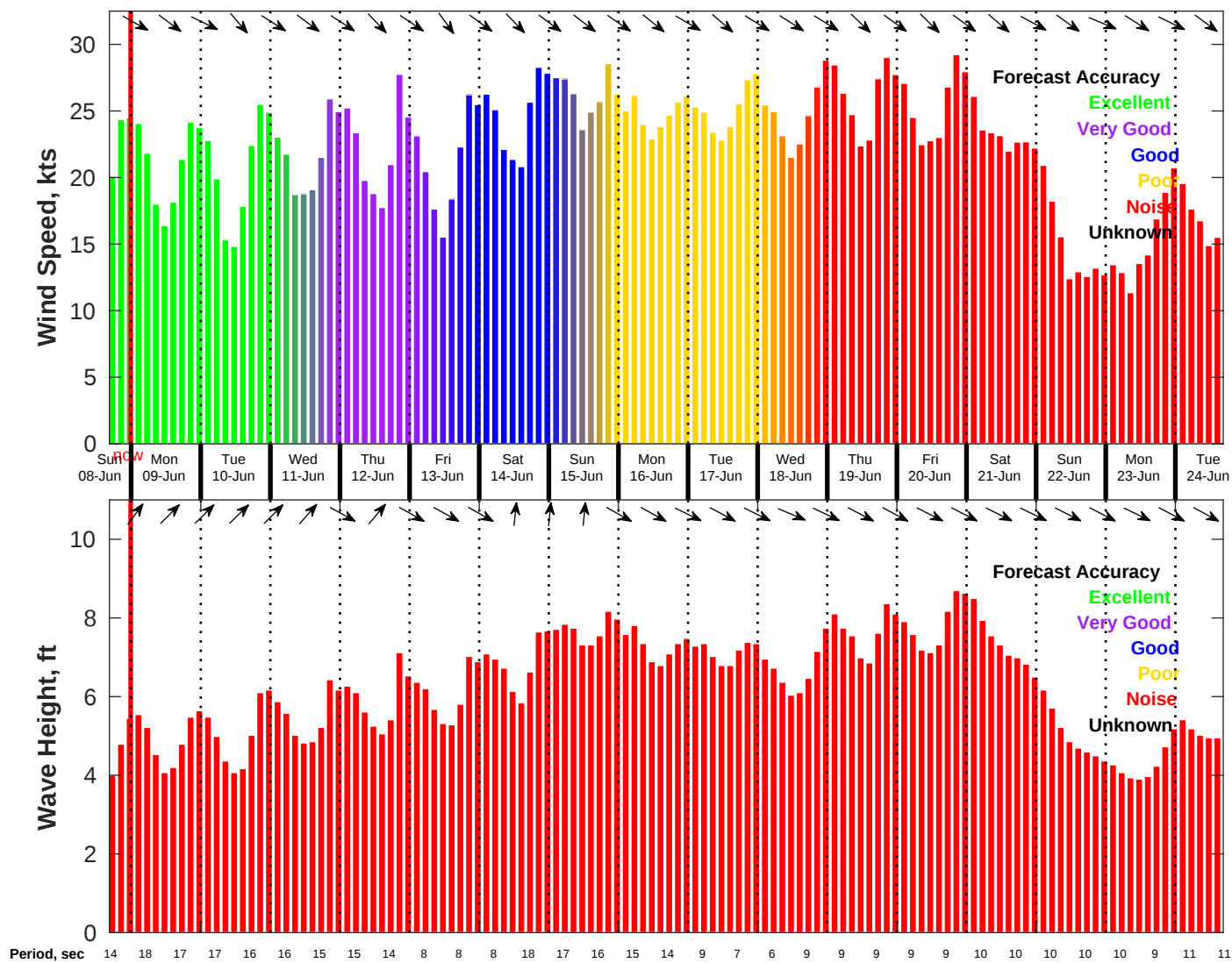
Wind & Wave Forecast for NDBC 46069 from 08-Jun-2025 16:00:00 to 24-Jun-2025 16:00:00
