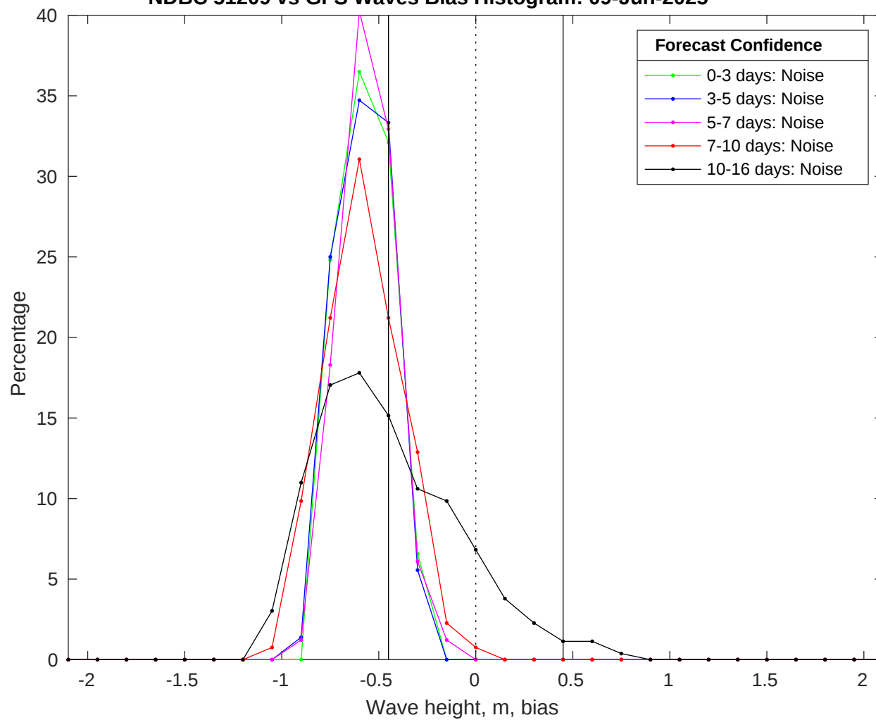
NDBC 51209 vs GFS Waves Bias Histogram: 09-Jun-2025
