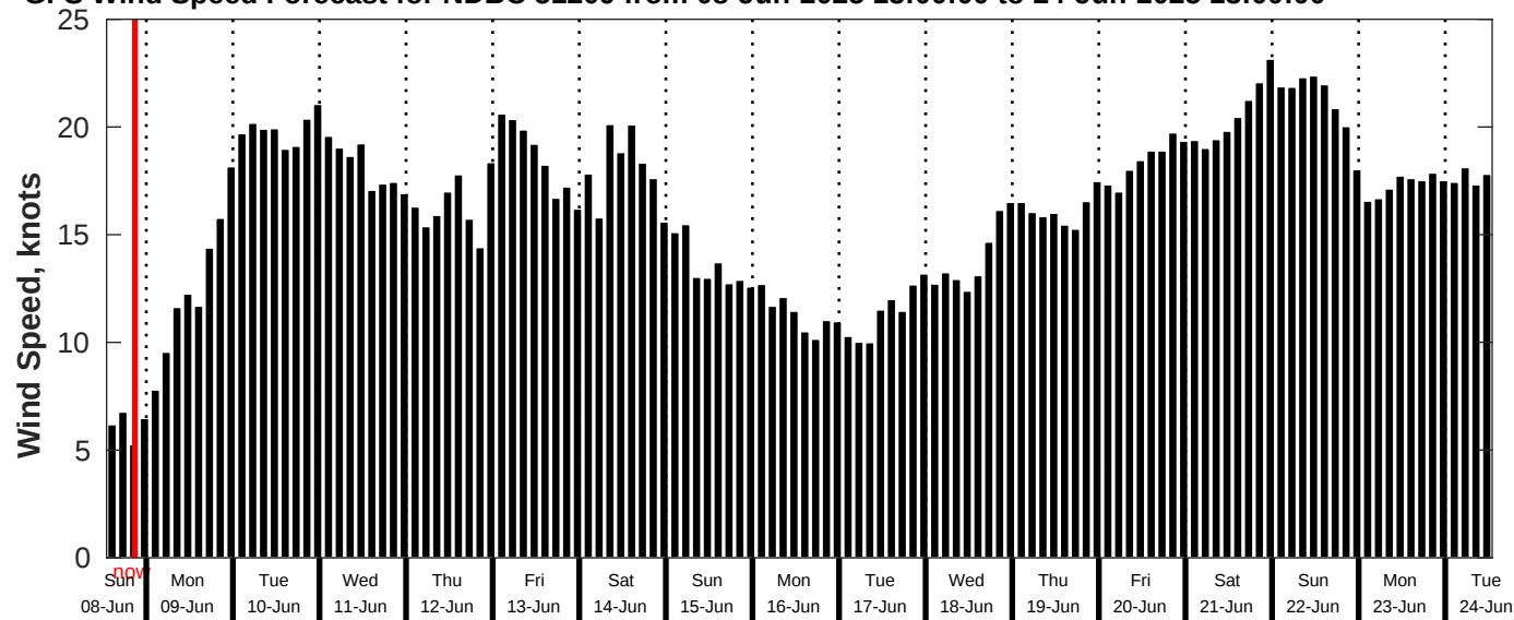
GFS Wind Speed Forecast for NDBC 51209 from 08-Jun-2025 13:00:00 to 24-Jun-2025 13:00:00
