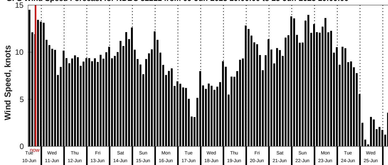
GFS Wind Speed Forecast for NDBC 52211 from 09-Jun-2025 10:00:00 to 25-Jun-2025 10:00:00
