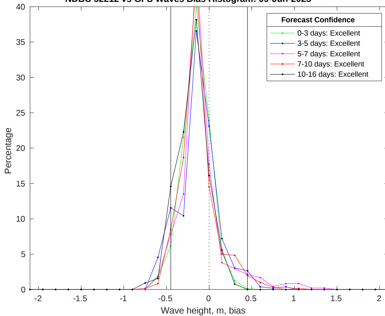
NDBC 52212 vs GFS Waves Bias Histogram: 09-Jun-2025
