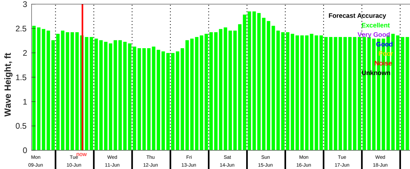
CMEMS Wave Forecast for NDBC 52212 from 08-Jun-2025 09:00:00 to 18-Jun-2025 09:00:00
