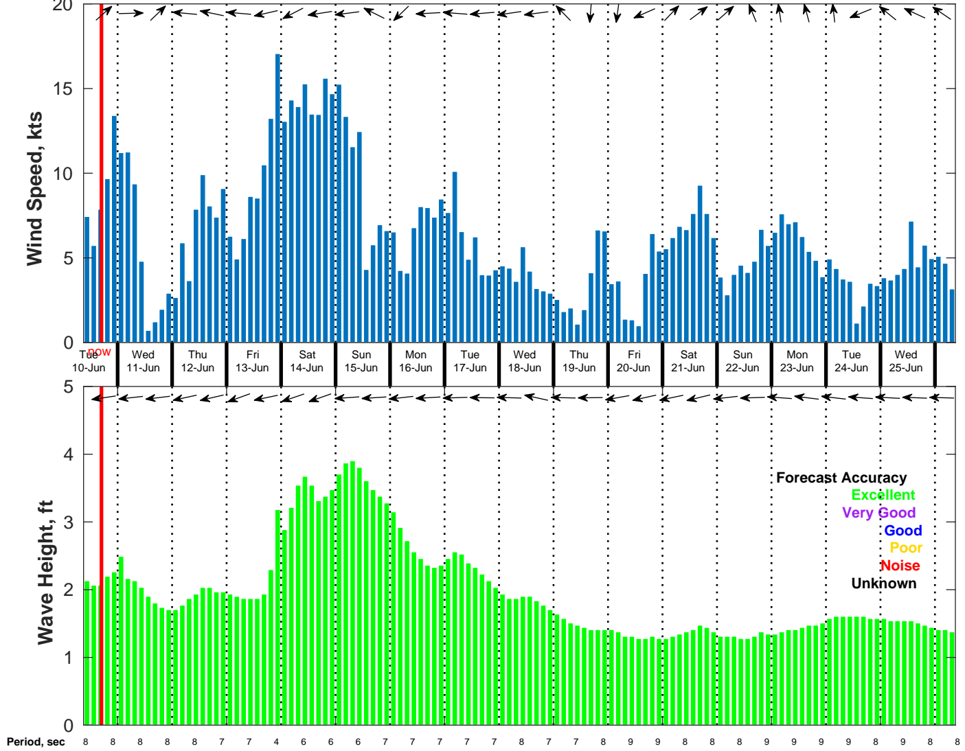
Wind & Wave Forecast for NDBC 52212 from 09-Jun-2025 09:00:00 to 25-Jun-2025 09:00:00
