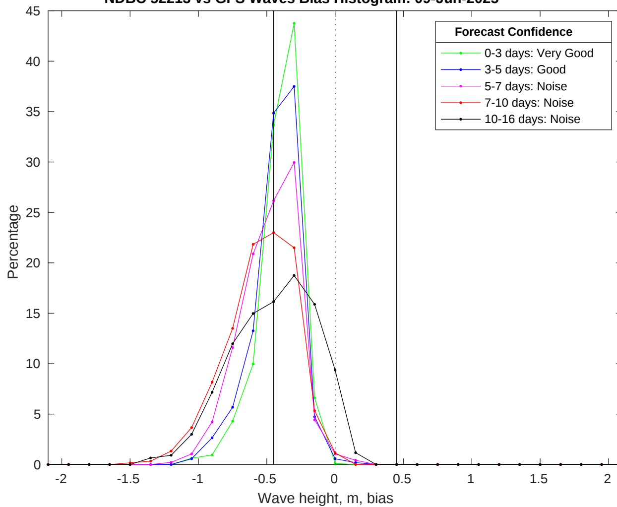
NDBC 52213 vs GFS Waves Bias Histogram: 09-Jun-2025
