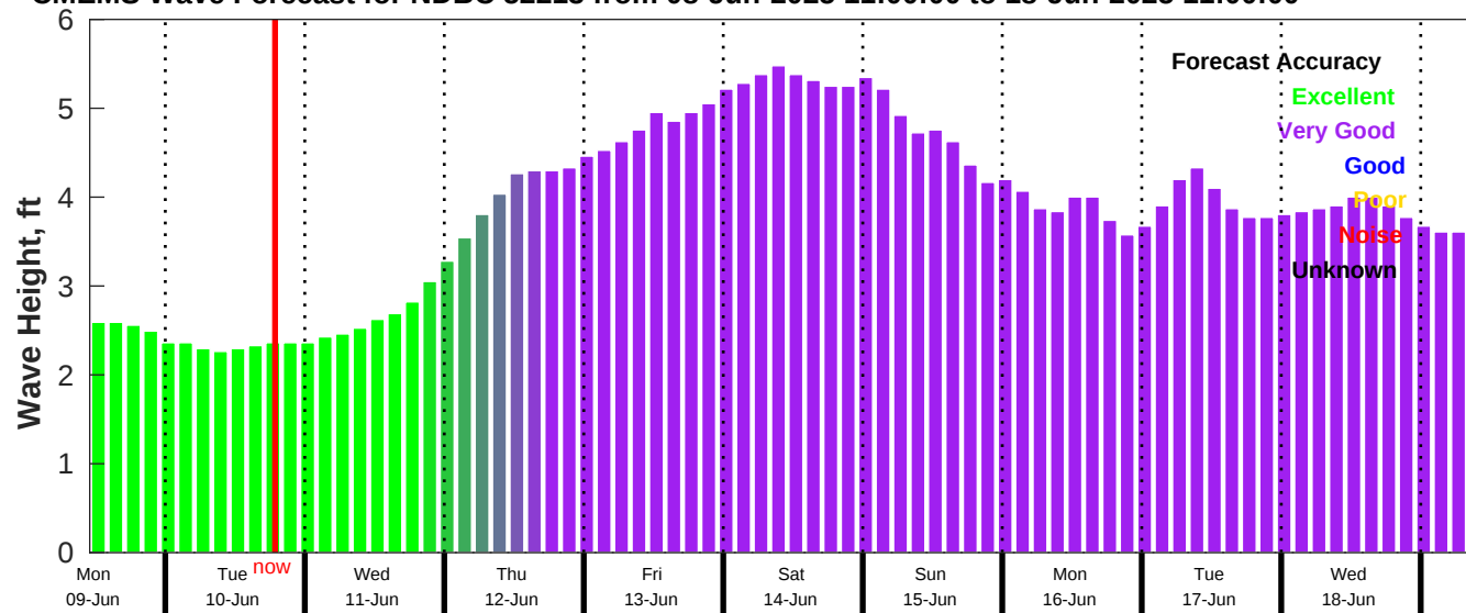
CMEMS Wave Forecast for NDBC 52213 from 08-Jun-2025 11:00:00 to 18-Jun-2025 11:00:00
