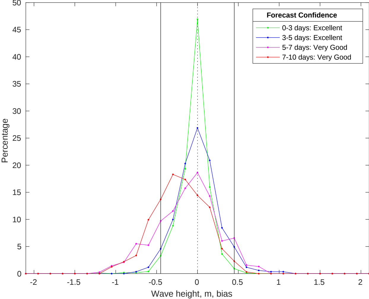
NDBC 41004 vs CMEMS Waves Bias Histogram: 10-Jun-2025
