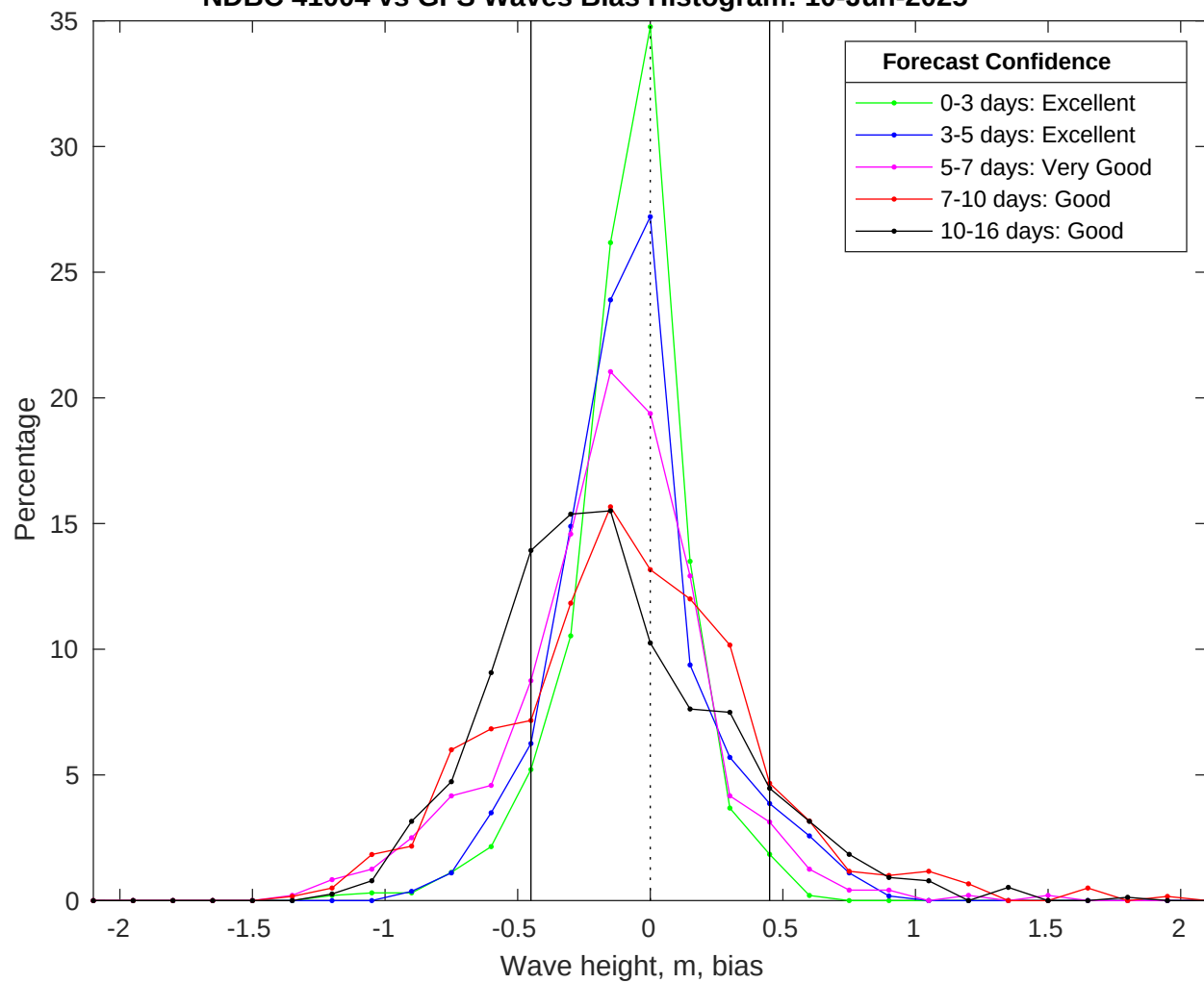
NDBC 41004 vs GFS Waves Bias Histogram: 10-Jun-2025
