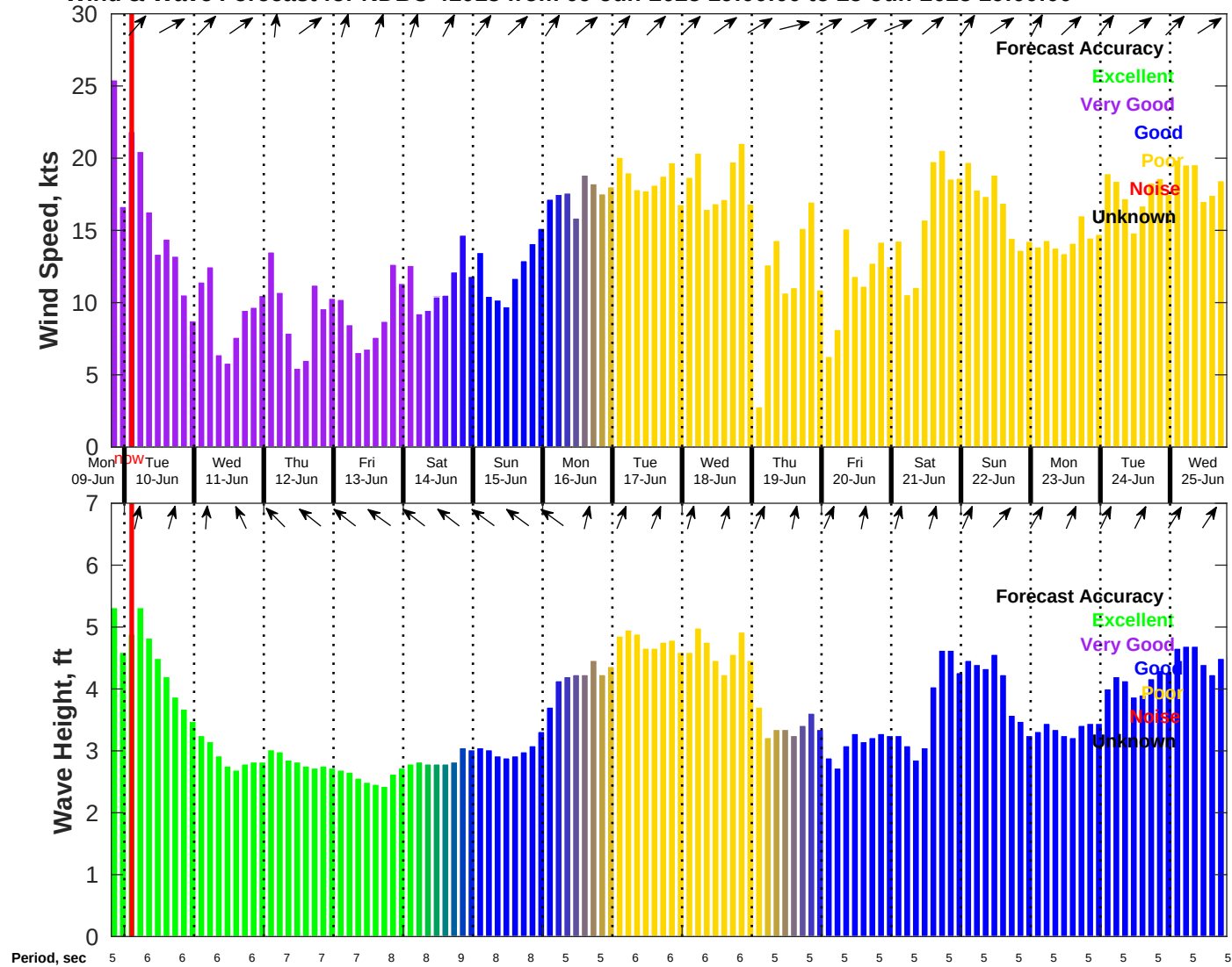
Wind & Wave Forecast for NDBC 41013 from 09-Jun-2025 19:00:00 to 25-Jun-2025 19:00:00
