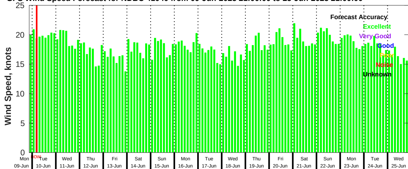
GFS Wind Speed Forecast for NDBC 41040 from 09-Jun-2025 21:00:00 to 25-Jun-2025 21:00:00
