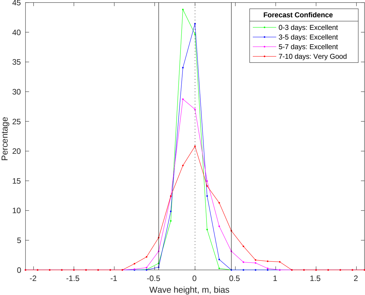
NDBC 42019 vs CMEMS Waves Bias Histogram: 10-Jun-2025
