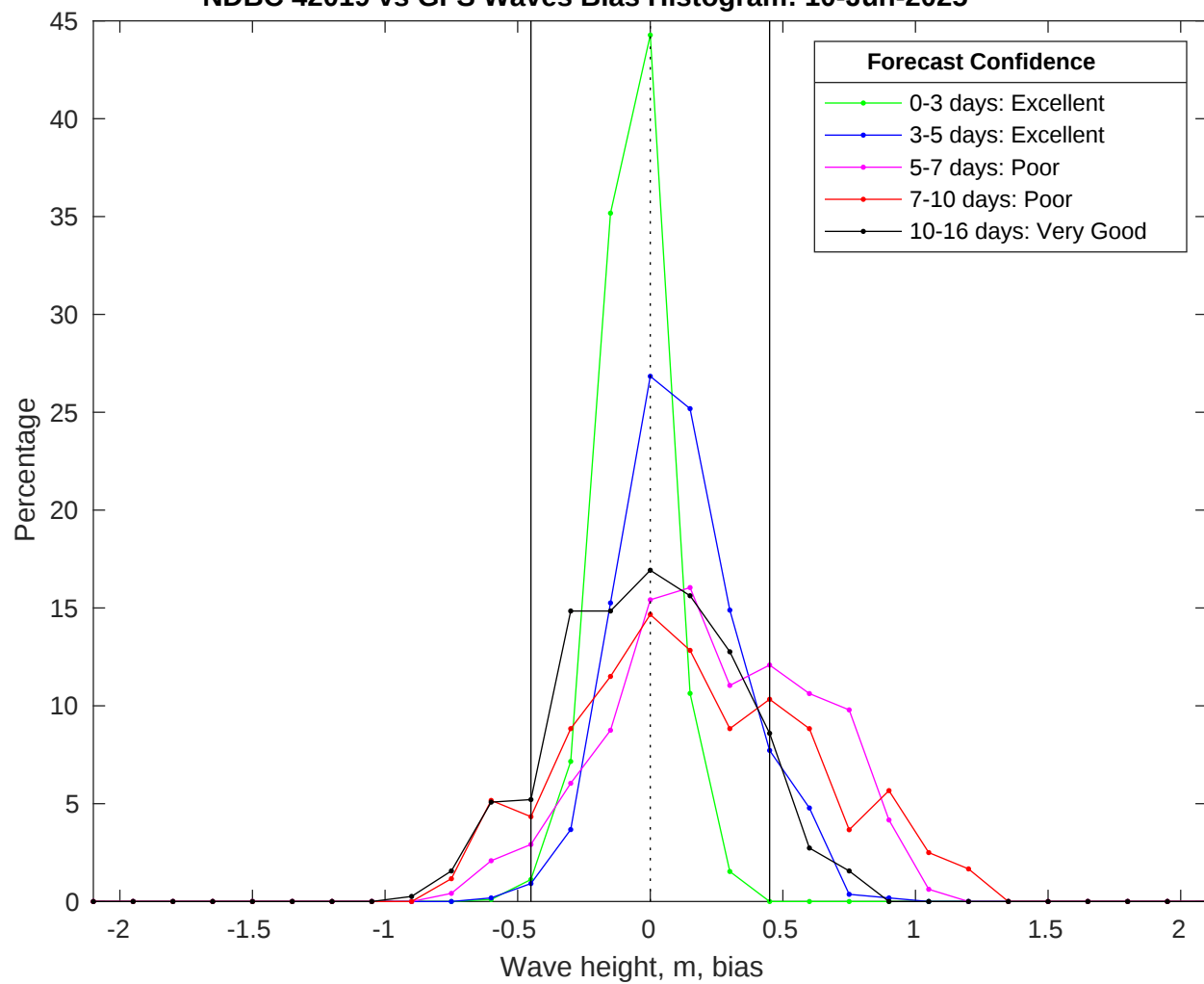
NDBC 42019 vs GFS Waves Bias Histogram: 10-Jun-2025
