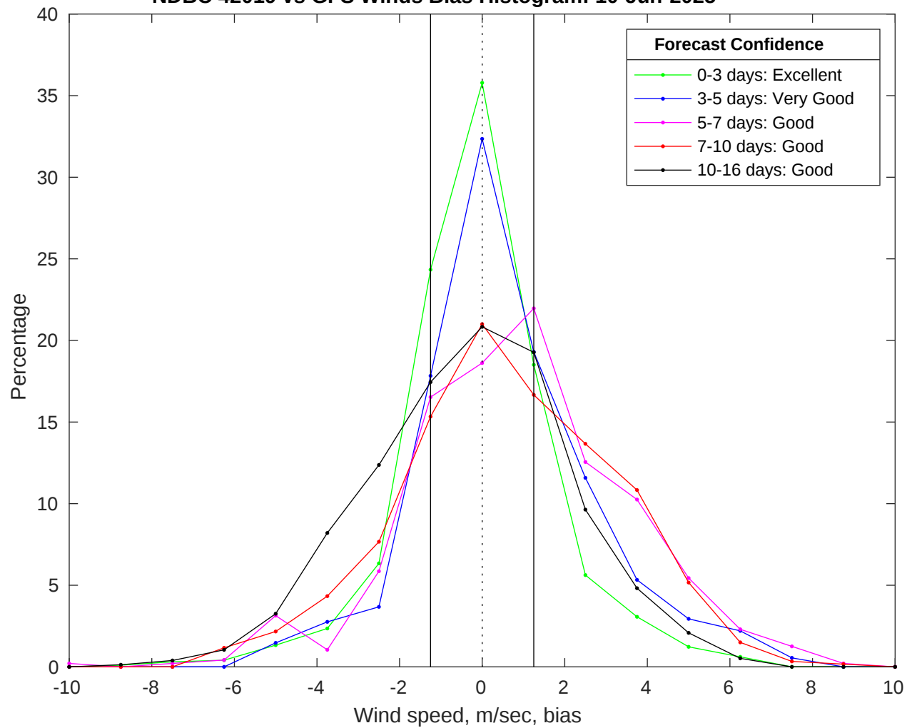
NDBC 42019 vs GFS Winds Bias Histogram: 10-Jun-2025
