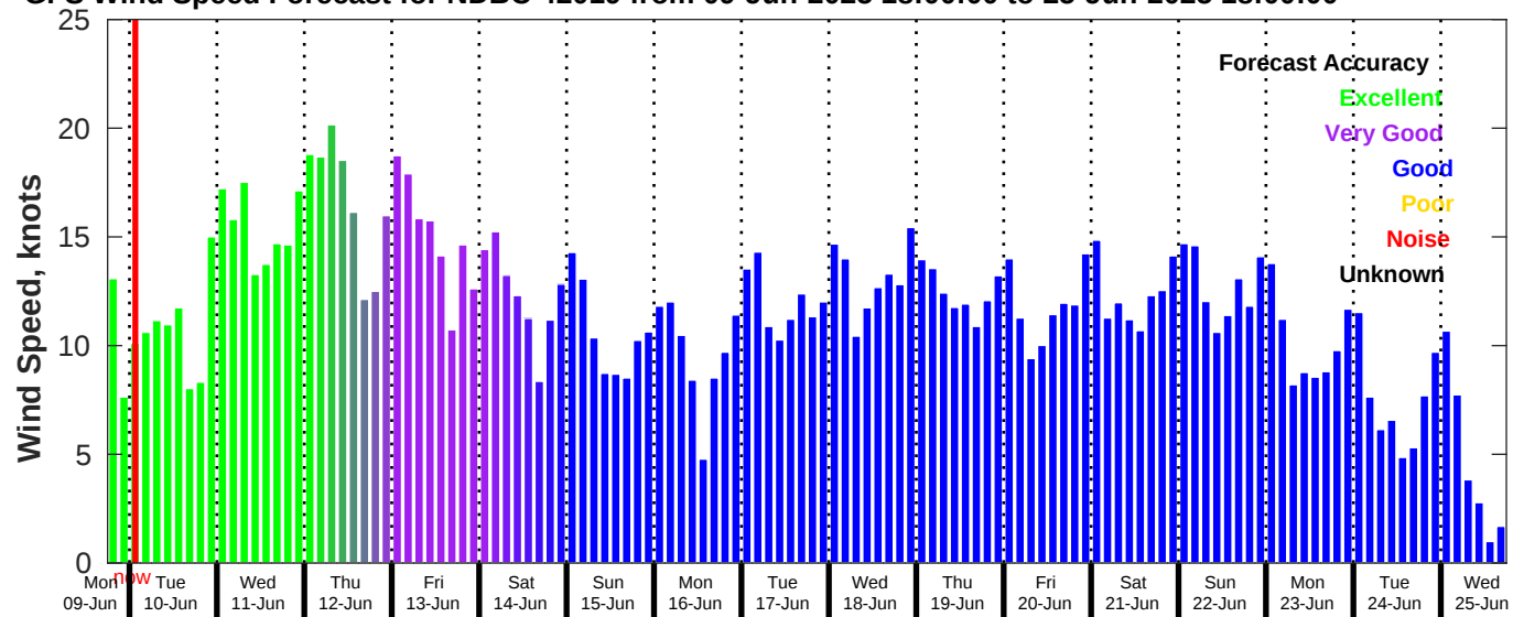
GFS Wind Speed Forecast for NDBC 42019 from 09-Jun-2025 18:00:00 to 25-Jun-2025 18:00:00
