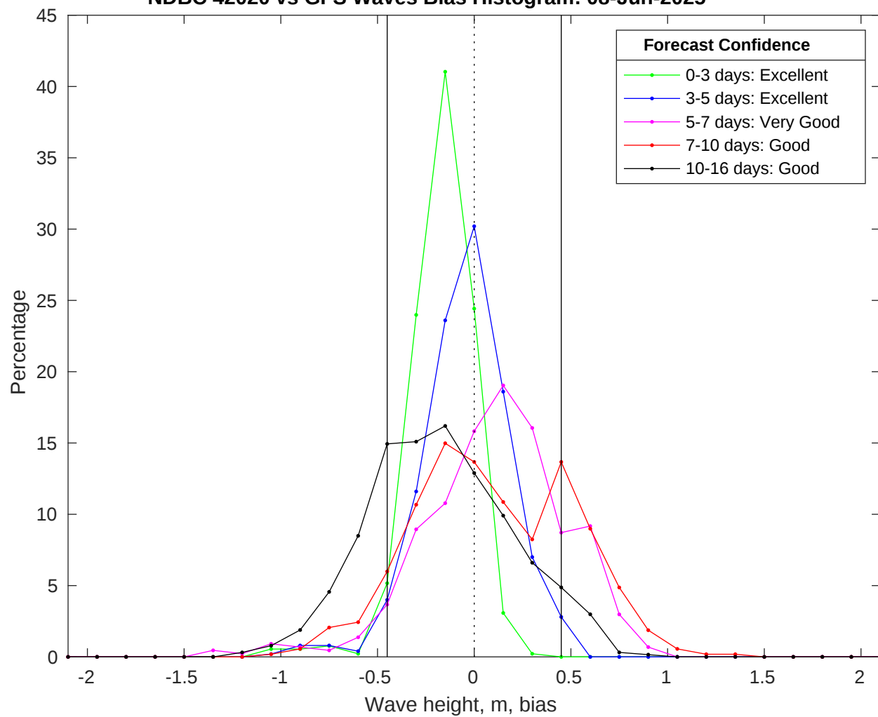
NDBC 42020 vs GFS Waves Bias Histogram: 08-Jun-2025
