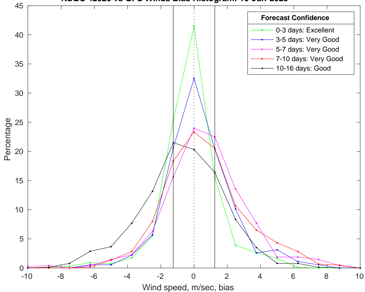
NDBC 42020 vs GFS Winds Bias Histogram: 10-Jun-2025
