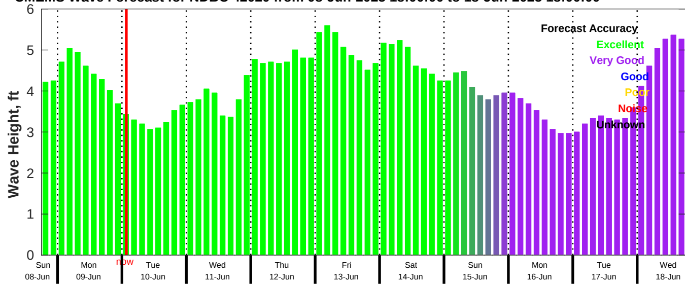
CMEMS Wave Forecast for NDBC 42020 from 08-Jun-2025 18:00:00 to 18-Jun-2025 18:00:00
