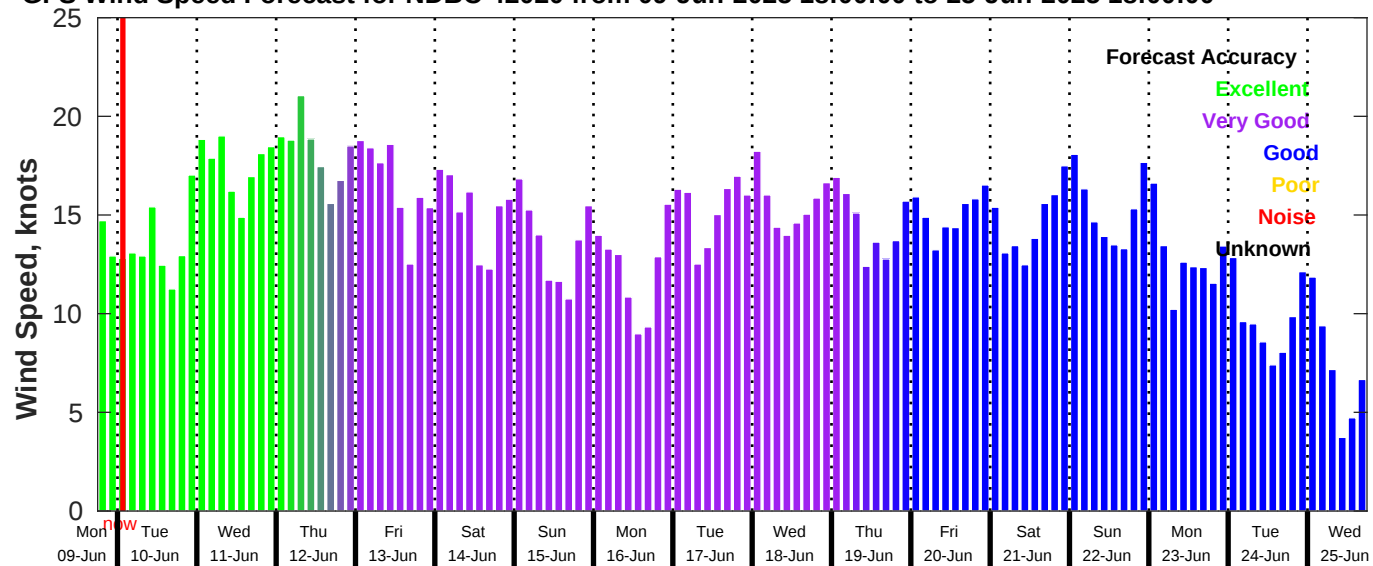
GFS Wind Speed Forecast for NDBC 42020 from 09-Jun-2025 18:00:00 to 25-Jun-2025 18:00:00
