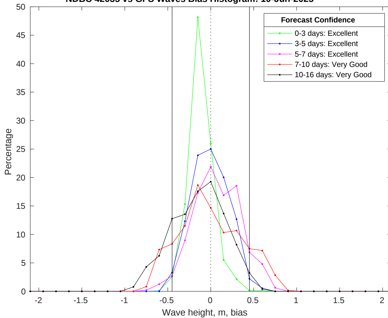
NDBC 42035 vs GFS Waves Bias Histogram: 10-Jun-2025
