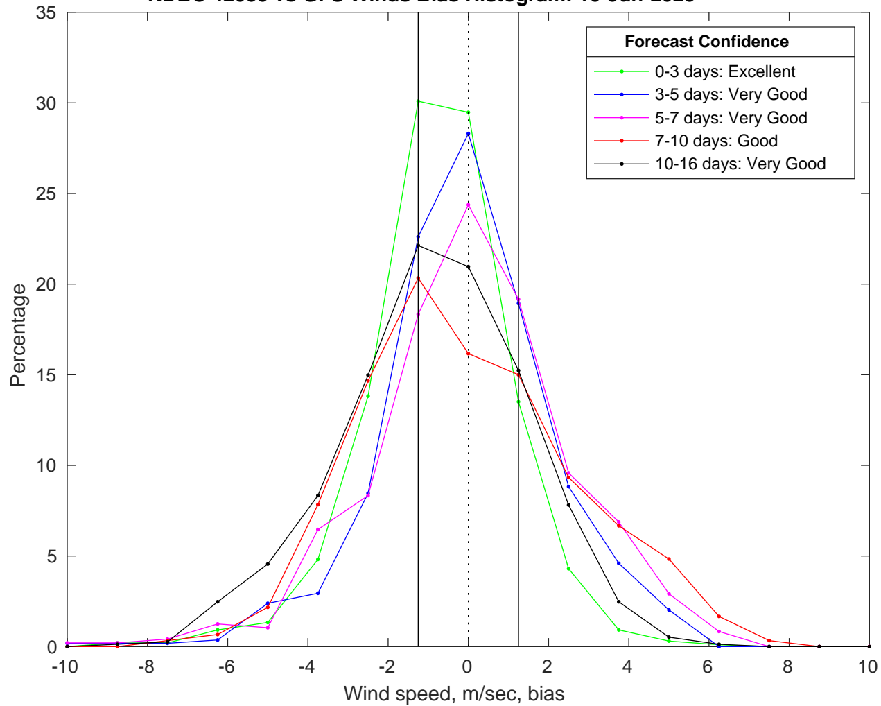
NDBC 42035 vs GFS Winds Bias Histogram: 10-Jun-2025
