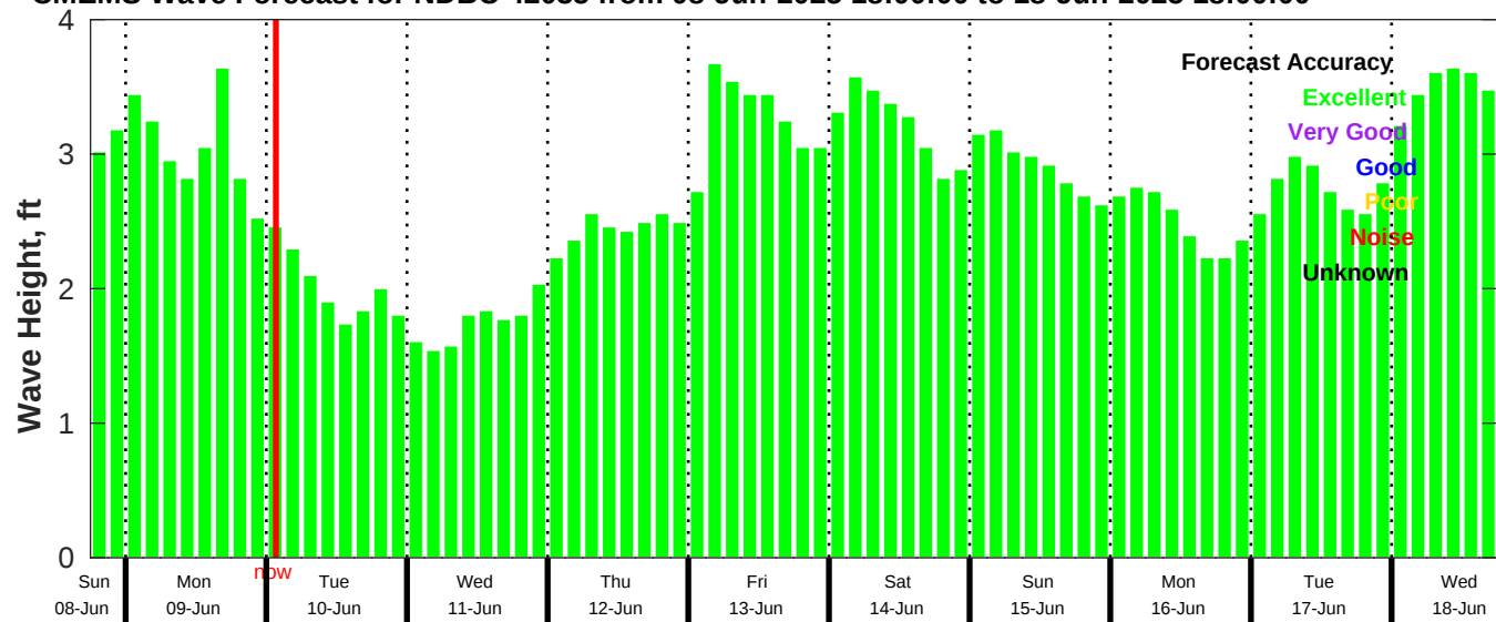
CMEMS Wave Forecast for NDBC 42035 from 08-Jun-2025 18:00:00 to 18-Jun-2025 18:00:00
