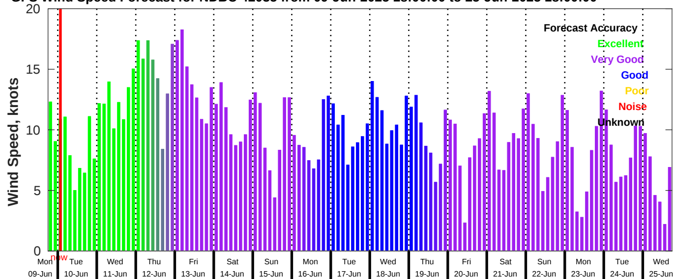
GFS Wind Speed Forecast for NDBC 42035 from 09-Jun-2025 18:00:00 to 25-Jun-2025 18:00:00
