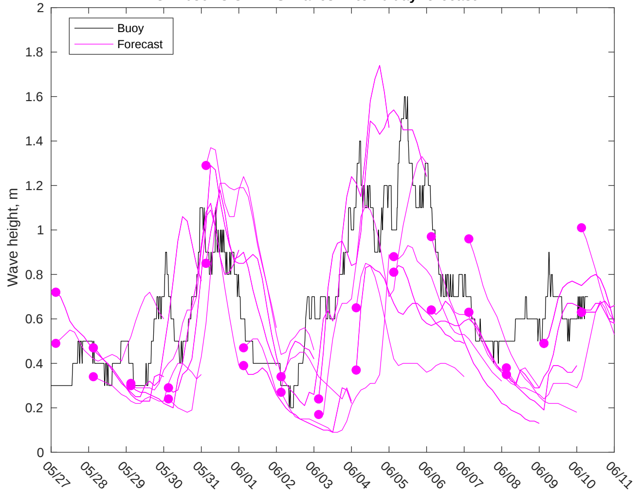
NDBC 42036 vs CMEMS Waves: 7 to 10 day forecast
