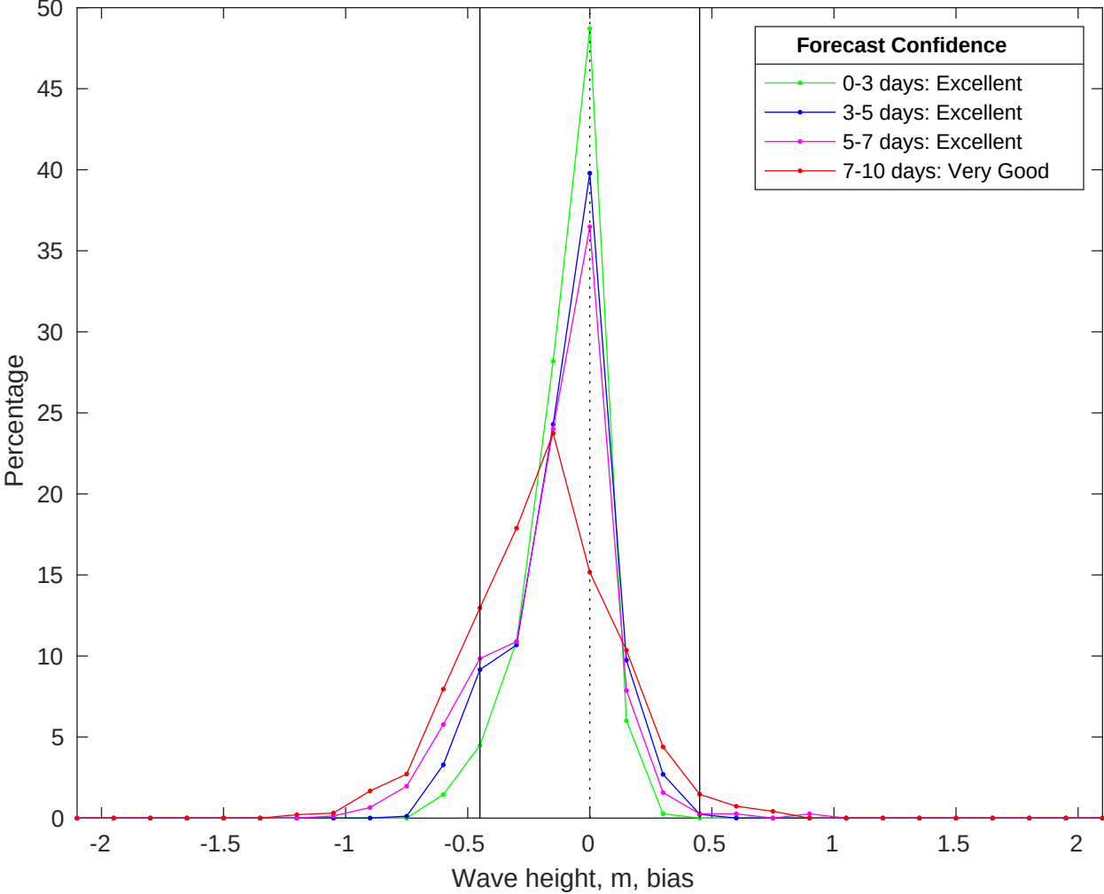
NDBC 42036 vs CMEMS Waves Bias Histogram: 10-Jun-2025
