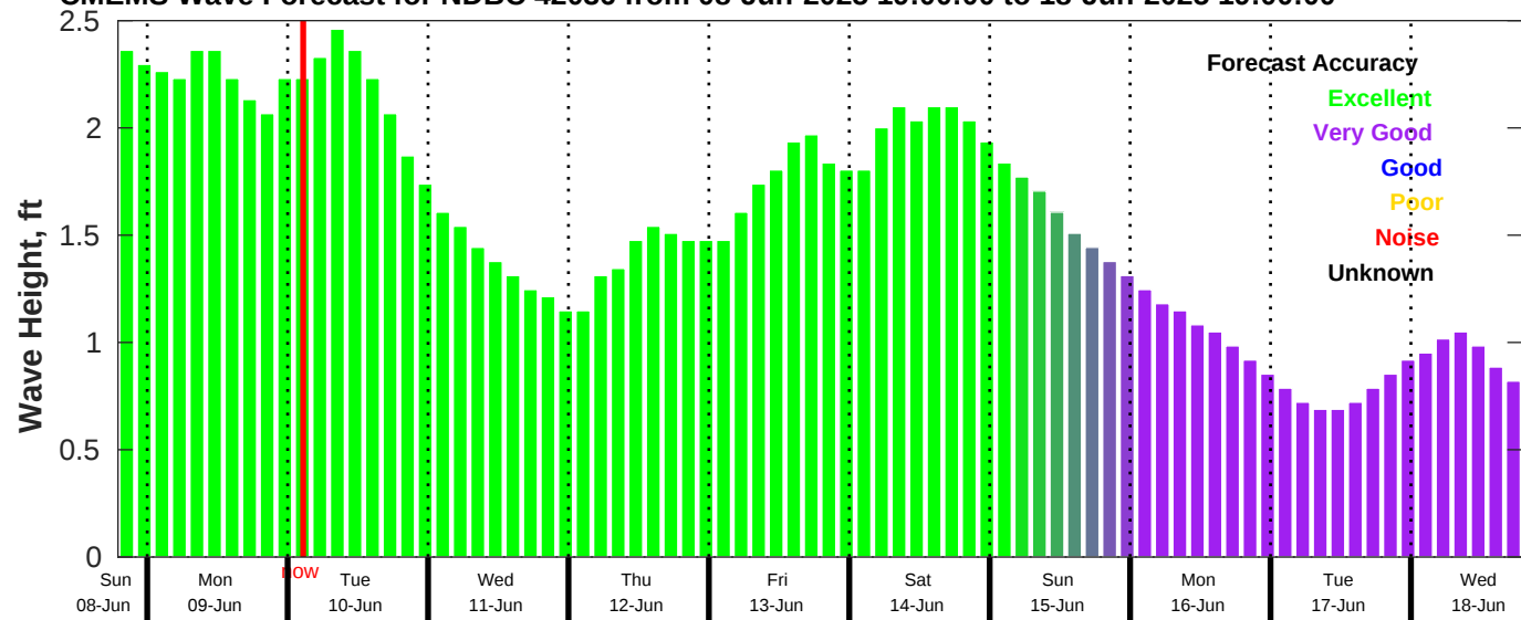
CMEMS Wave Forecast for NDBC 42036 from 08-Jun-2025 19:00:00 to 18-Jun-2025 19:00:00
