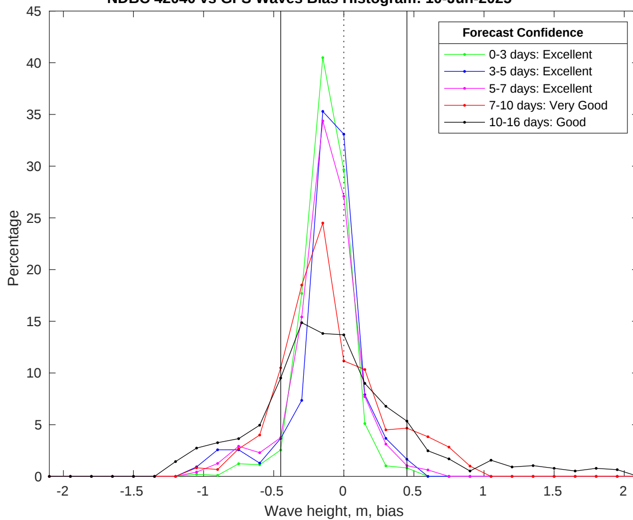
NDBC 42040 vs GFS Waves Bias Histogram: 10-Jun-2025
