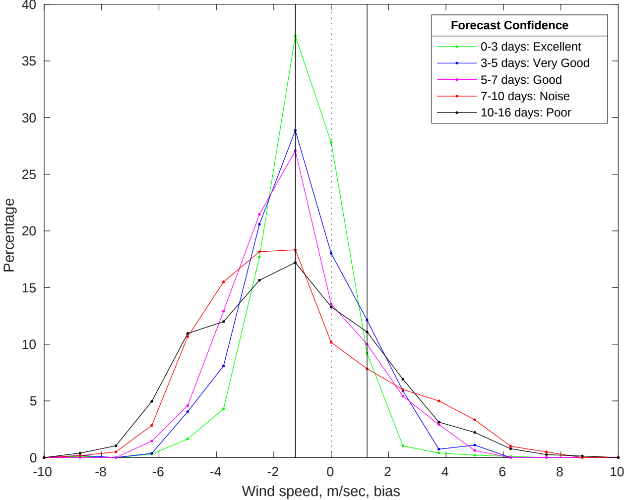
NDBC 42040 vs GFS Winds Bias Histogram: 10-Jun-2025
