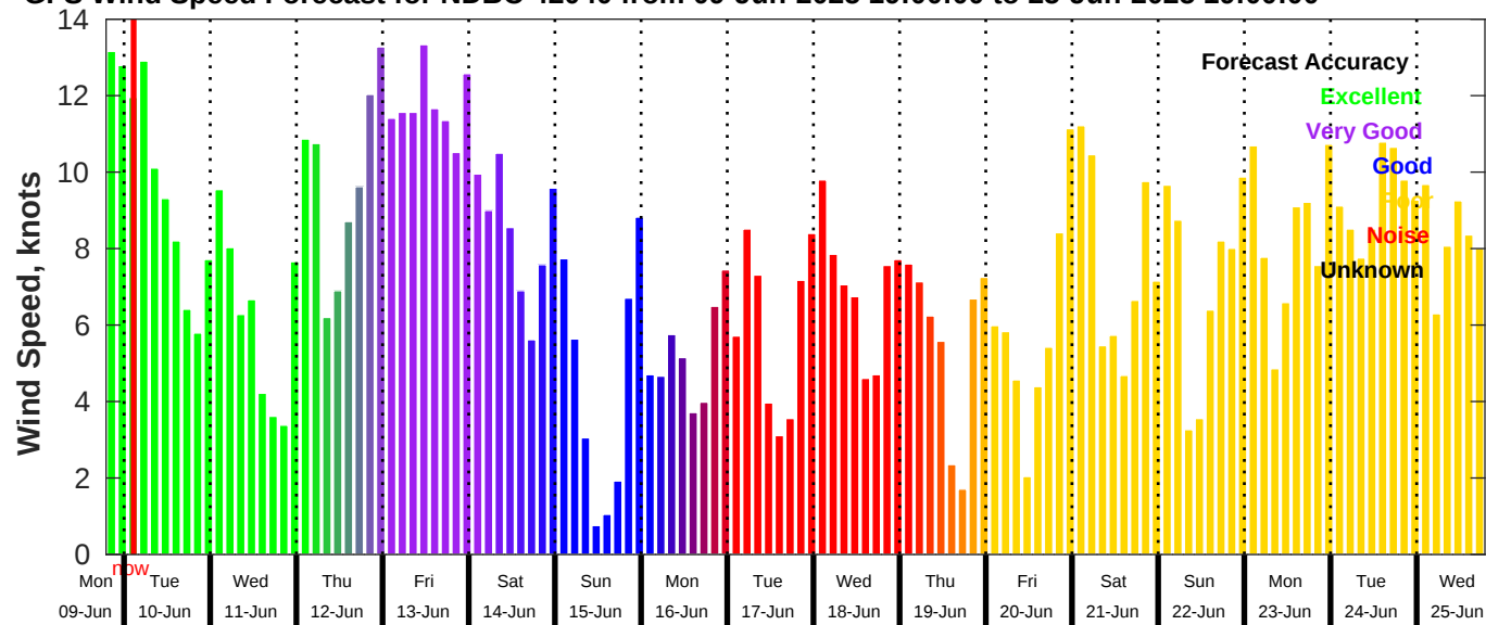
GFS Wind Speed Forecast for NDBC 42040 from 09-Jun-2025 19:00:00 to 25-Jun-2025 19:00:00
