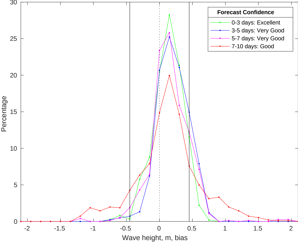
NDBC 46011 vs CMEMS Waves Bias Histogram: 10-Jun-2025
