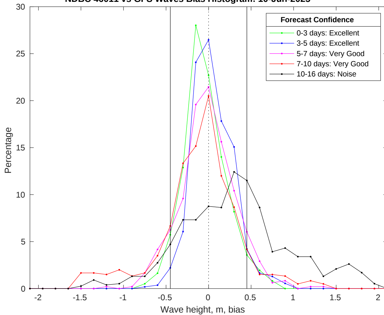
NDBC 46011 vs GFS Waves Bias Histogram: 10-Jun-2025
