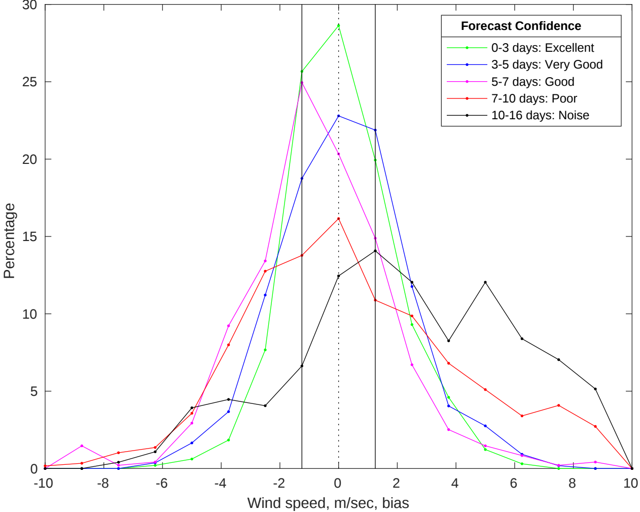
NDBC 46011 vs GFS Winds Bias Histogram: 10-Jun-2025
