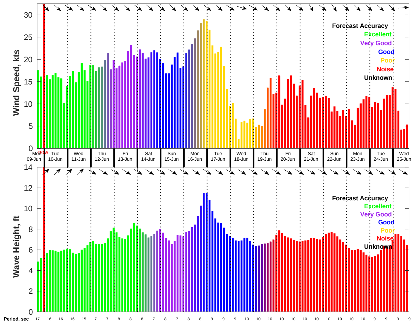
Wind & Wave Forecast for NDBC 46011 from 09-Jun-2025 16:00:00 to 25-Jun-2025 16:00:00
