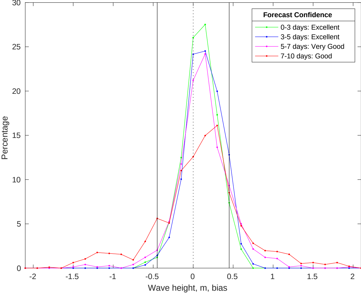
NDBC 46028 vs CMEMS Waves Bias Histogram: 10-Jun-2025
