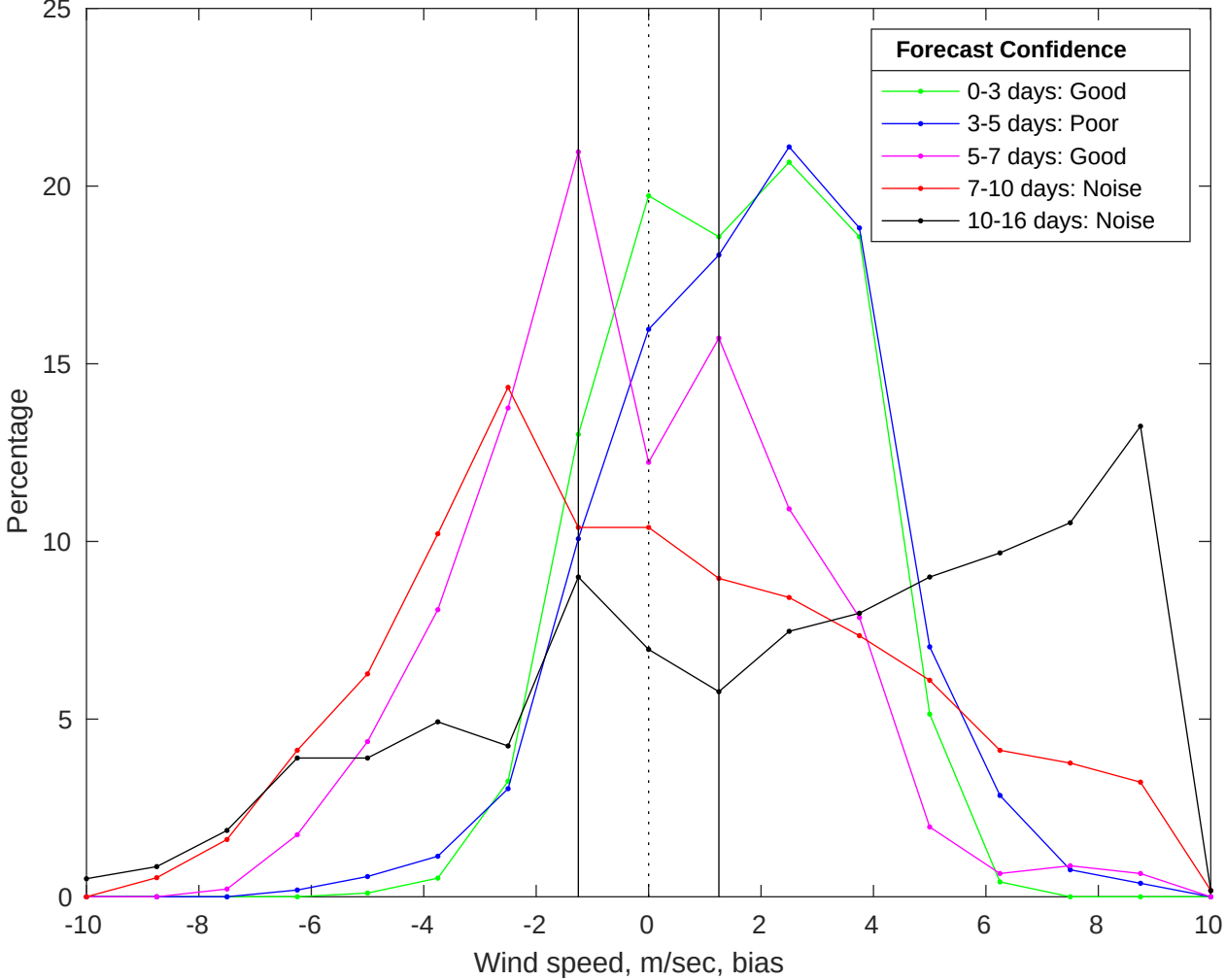
NDBC 46028 vs GFS Winds Bias Histogram: 10-Jun-2025
