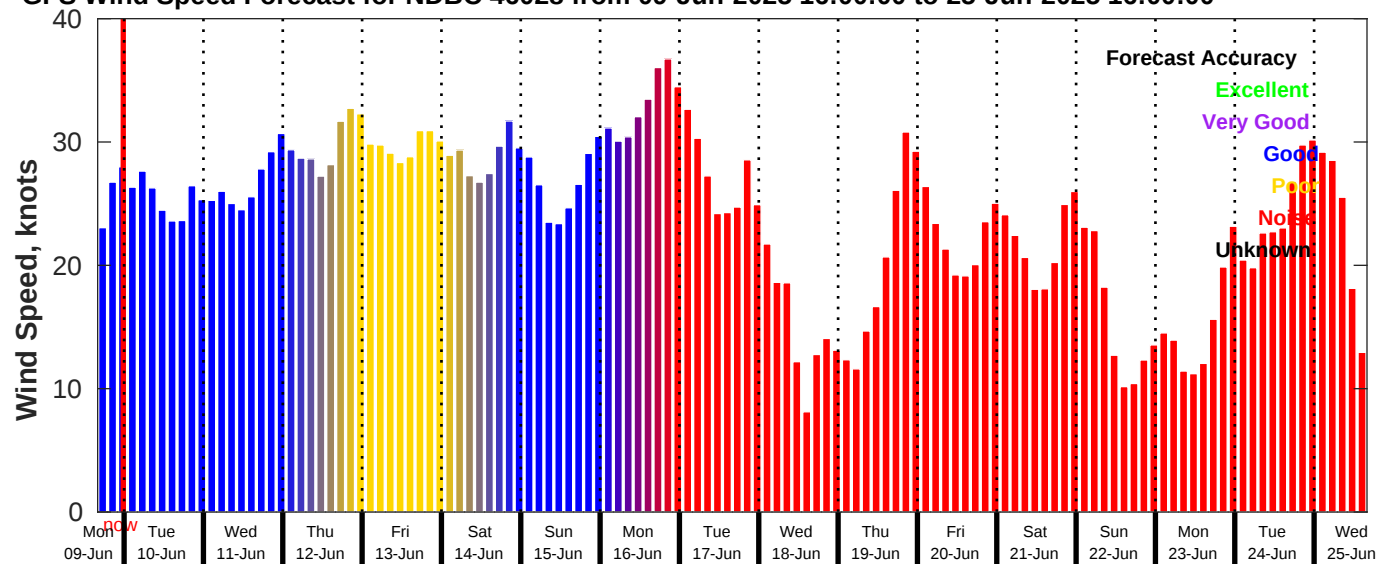
GFS Wind Speed Forecast for NDBC 46028 from 09-Jun-2025 16:00:00 to 25-Jun-2025 16:00:00
