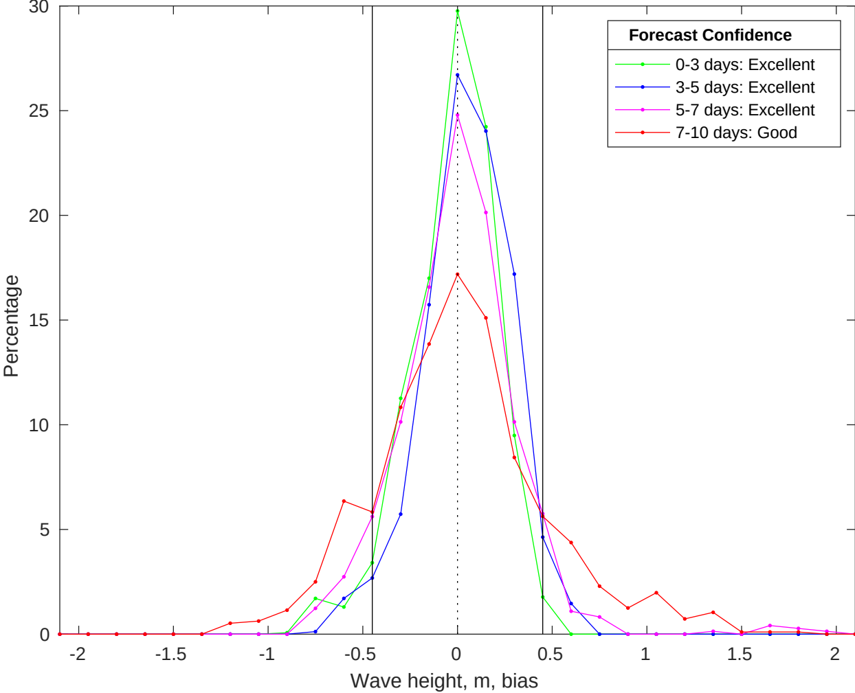
NDBC 46054 vs CMEMS Waves Bias Histogram: 10-Jun-2025
