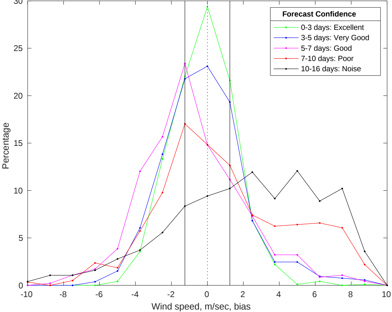
NDBC 46054 vs GFS Winds Bias Histogram: 10-Jun-2025
