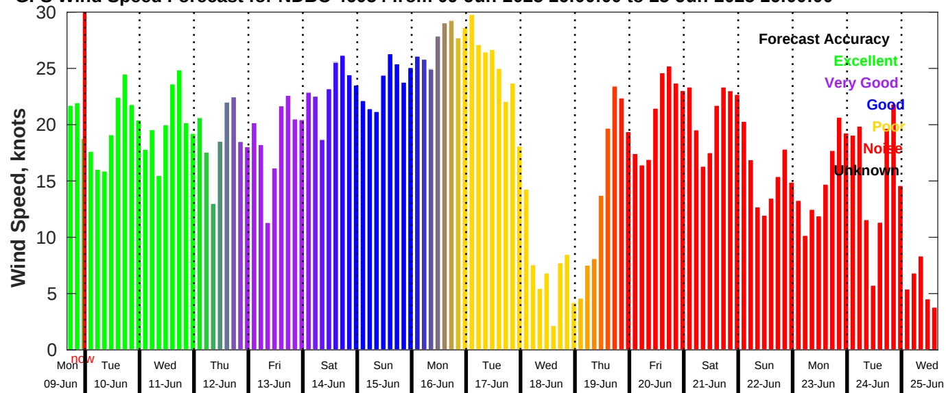
GFS Wind Speed Forecast for NDBC 46054 from 09-Jun-2025 16:00:00 to 25-Jun-2025 16:00:00
