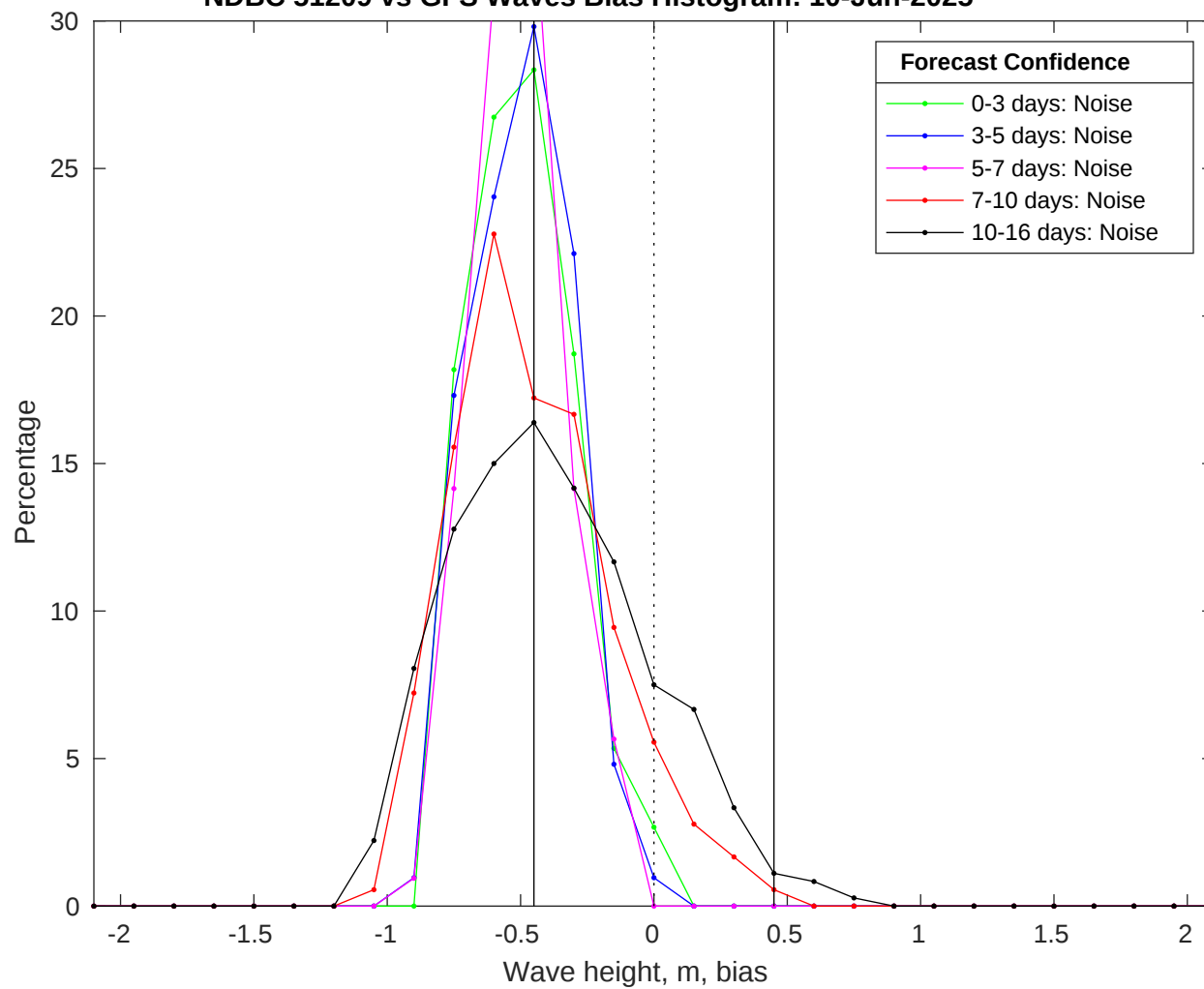
NDBC 51209 vs GFS Waves Bias Histogram: 10-Jun-2025
