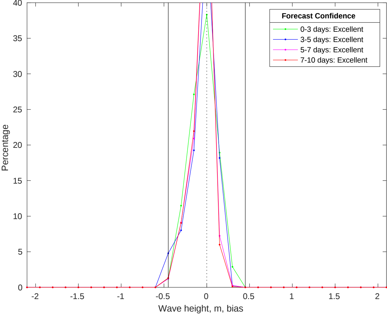
NDBC 52212 vs CMEMS Waves Bias Histogram: 10-Jun-2025
