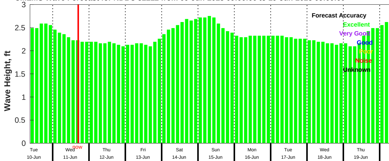
CMEMS Wave Forecast for NDBC 52212 from 09-Jun-2025 09:00:00 to 19-Jun-2025 09:00:00
