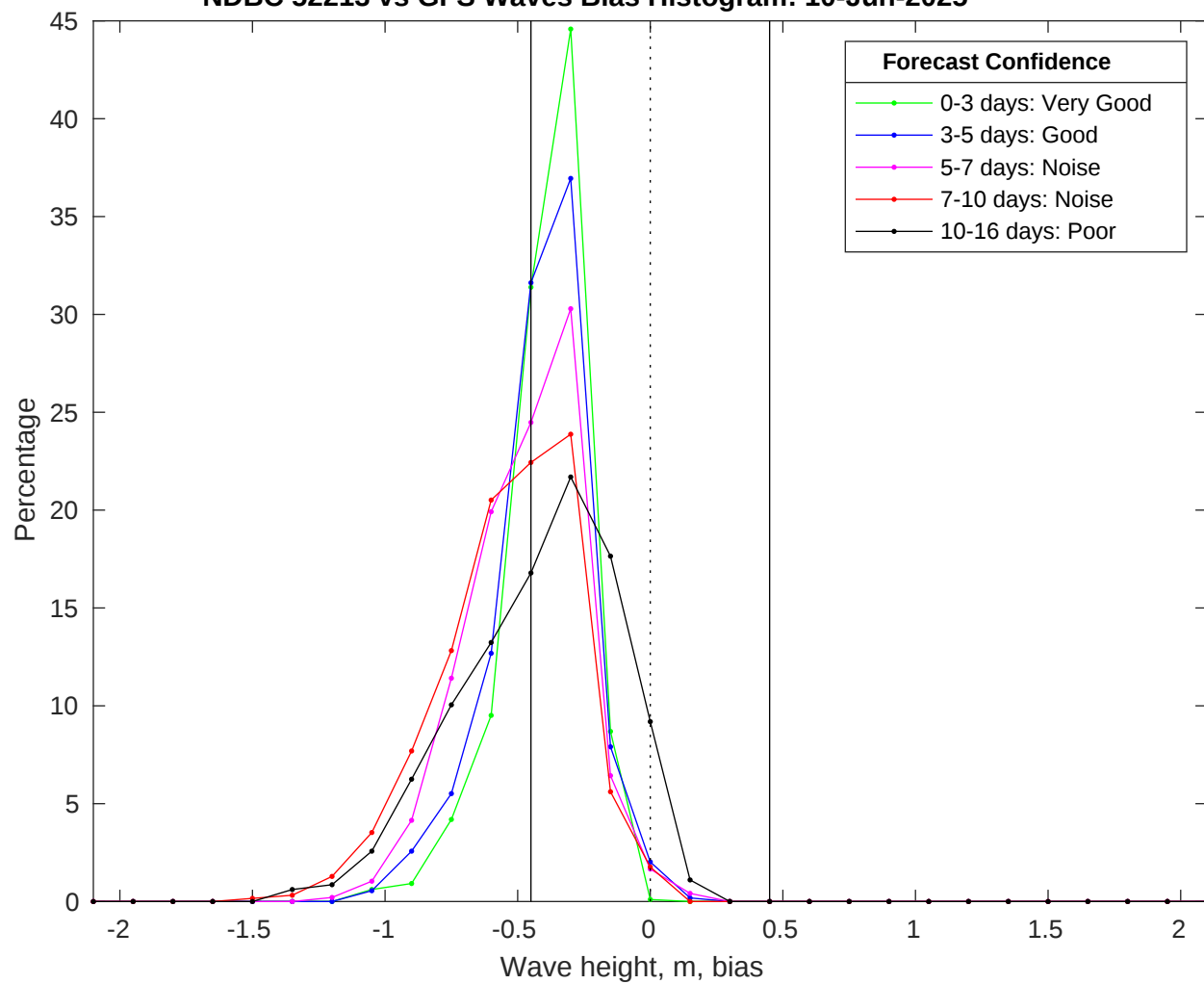
NDBC 52213 vs GFS Waves Bias Histogram: 10-Jun-2025
