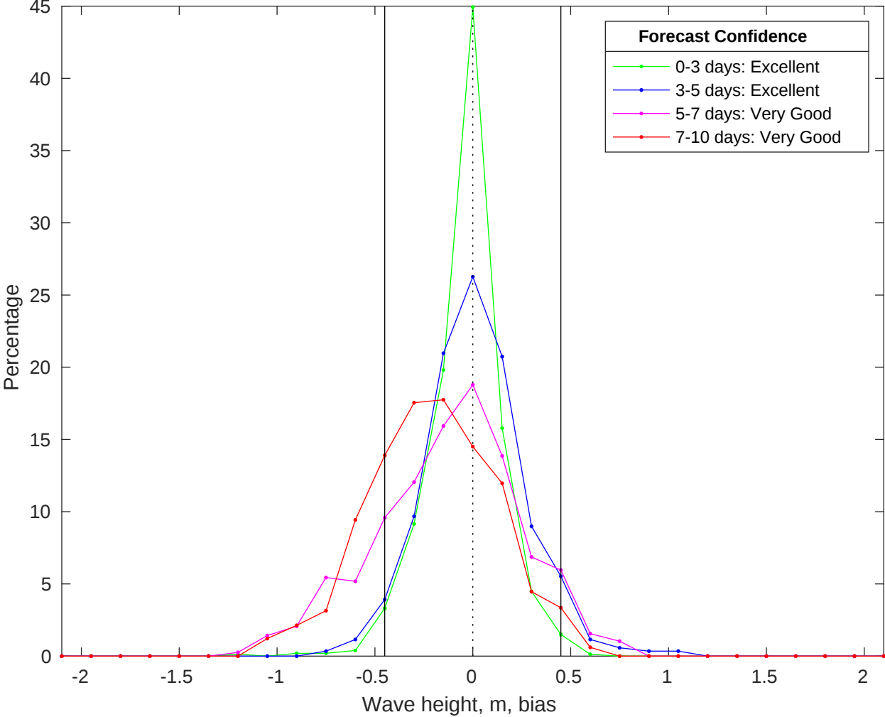
NDBC 41004 vs CMEMS Waves Bias Histogram: 11-Jun-2025
