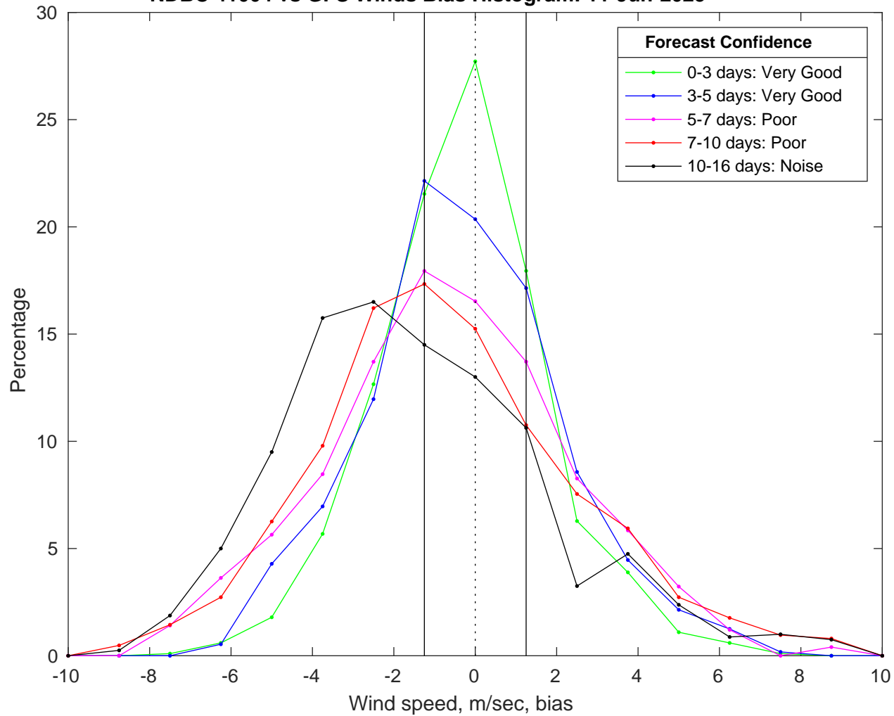
NDBC 41004 vs GFS Winds Bias Histogram: 11-Jun-2025
