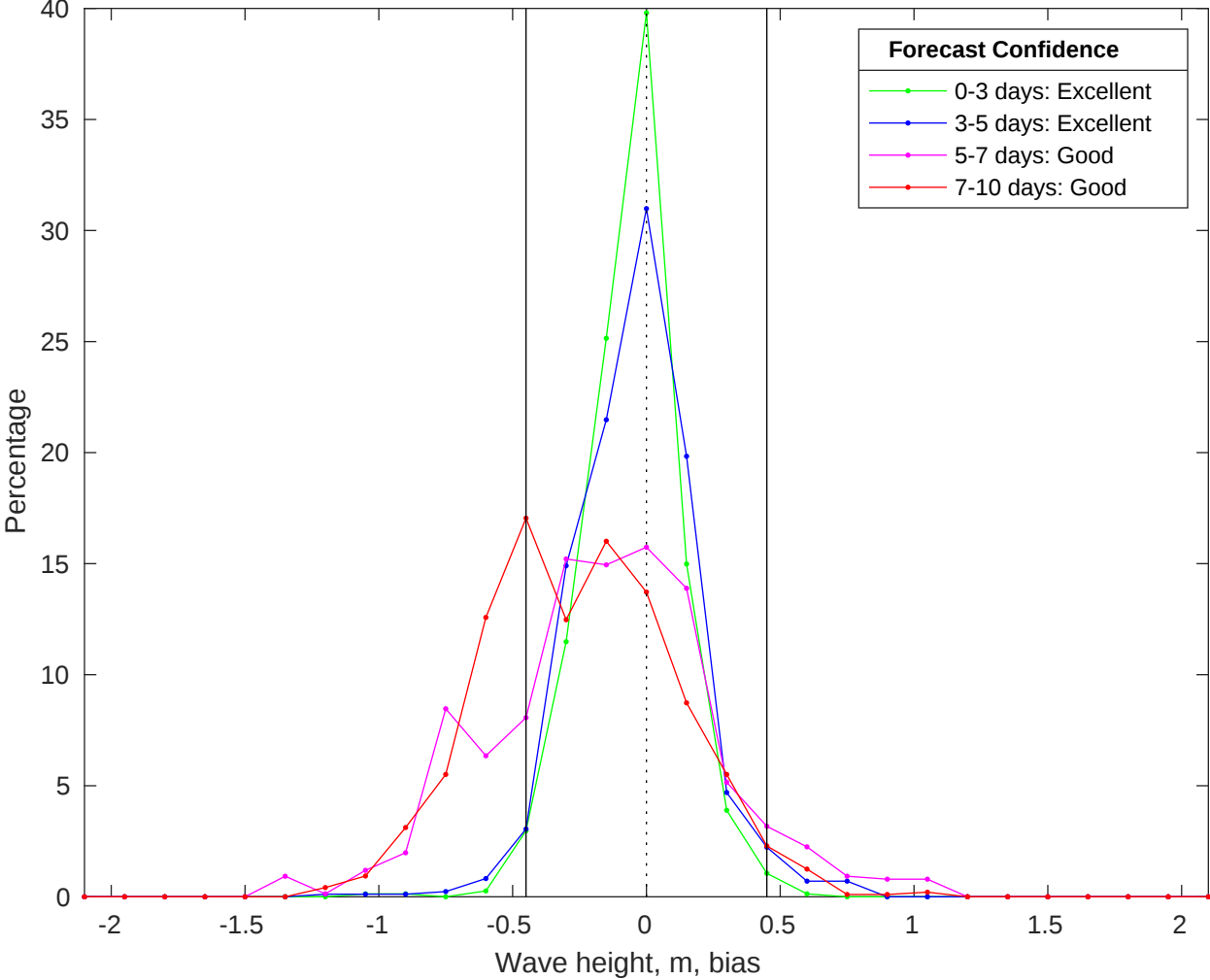
NDBC 41013 vs CMEMS Waves Bias Histogram: 11-Jun-2025
