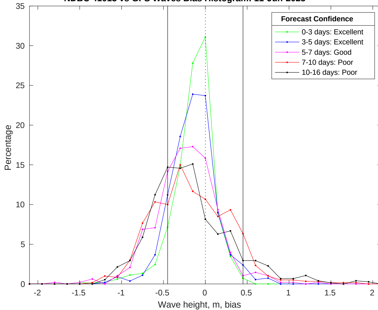
NDBC 41013 vs GFS Waves Bias Histogram: 11-Jun-2025
